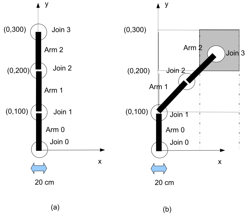
Figure 2: A 2D simplified robot arm.
